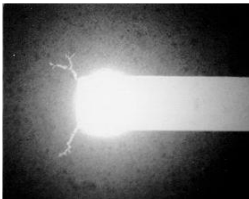
Fig. 9. Vicinal illumination view of corner crowding induced damage [1].
