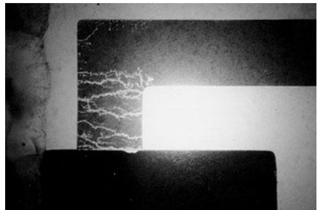
Fig. 11. Vicinal illumination view of transverse cracking typical of relatively high voltage ESD damage [1].
