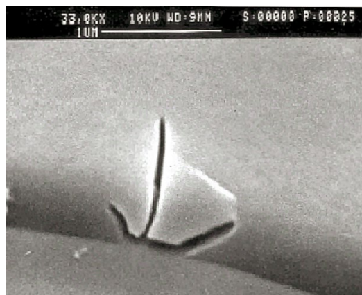
Figure 2. ESD damage to most semiconductors is often so subtle that it cannot be seen without very high magnification (image courtesy of Hi-Rel Laboratories).
