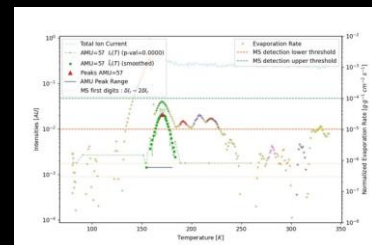
Single matched spectra for single species
