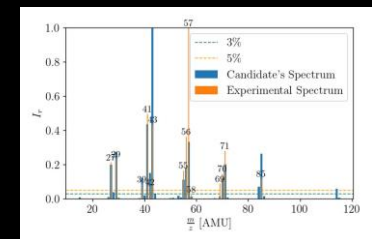
Ranking of all matched molecules
